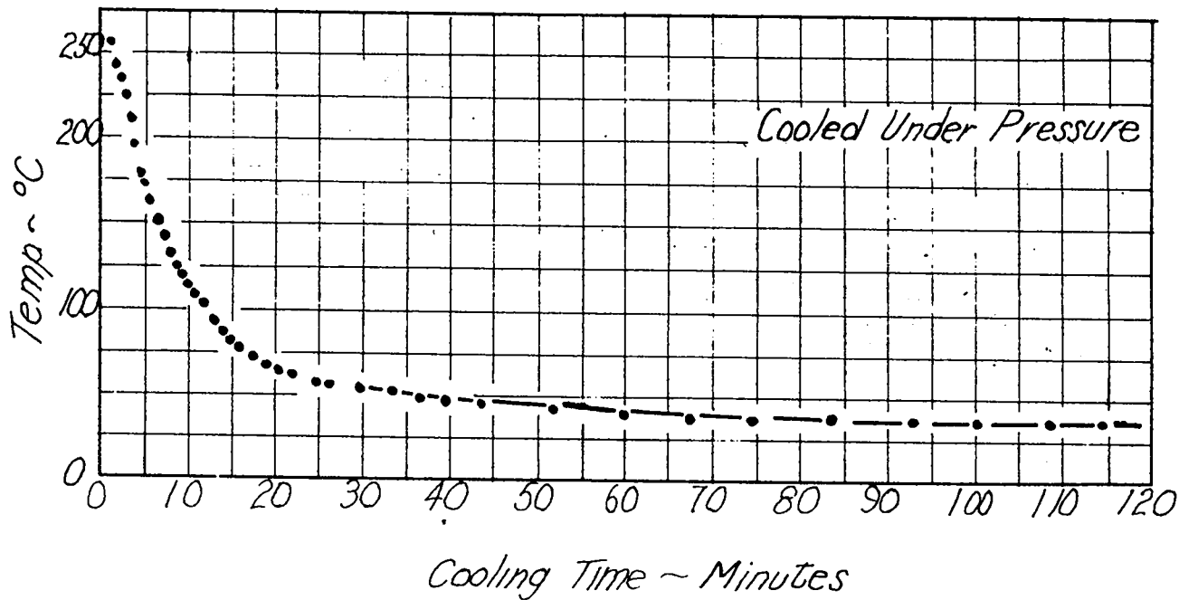
Fig. 5 Heating and Cooling Curves for Second 49 Hemisphere Pressing
